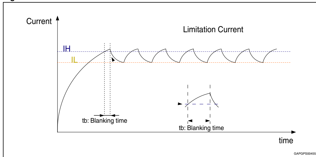
Figure 11. Current limitation
