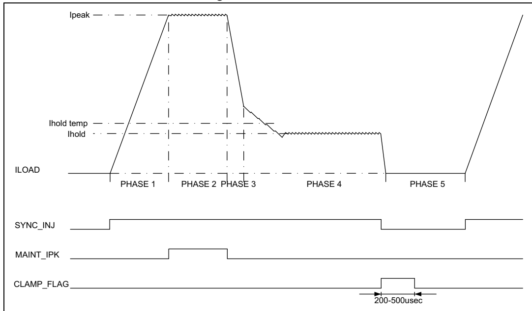
Figure 2. Waveforms
