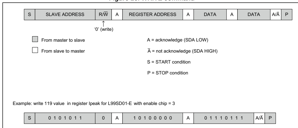
Figure 16. WRITE command
