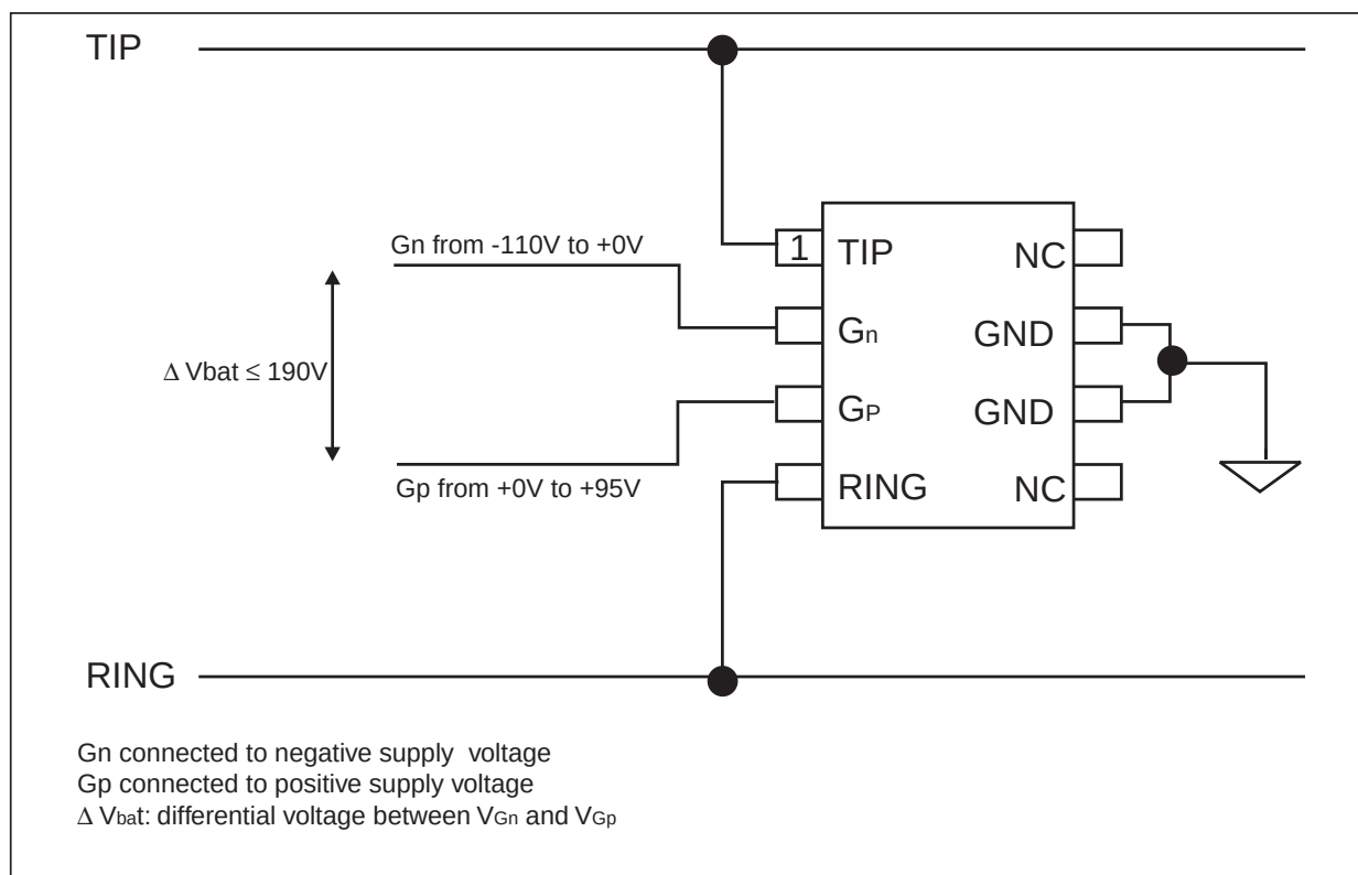
Fig. 1: Test circuit
