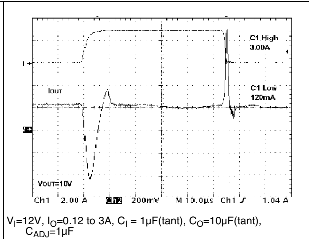
Figure 22. Load transient
