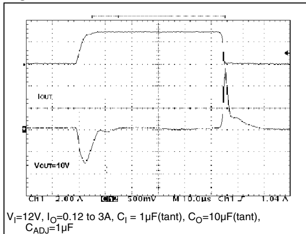
Figure 23. Load transient
