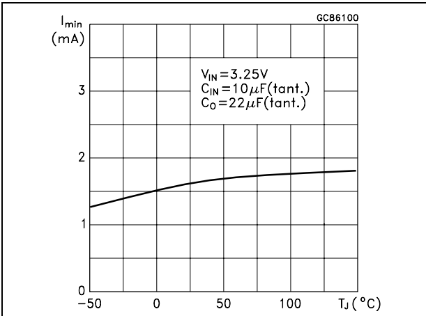
Figure 19. Stability
