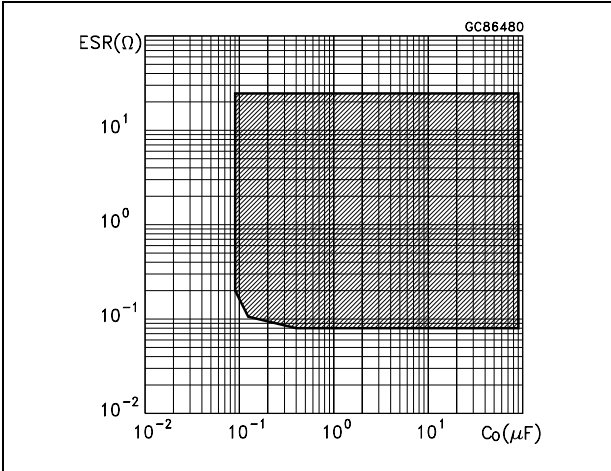
Figure 19. Stability
