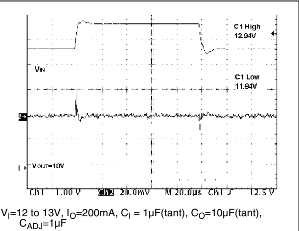
Figure 20. Line transient
