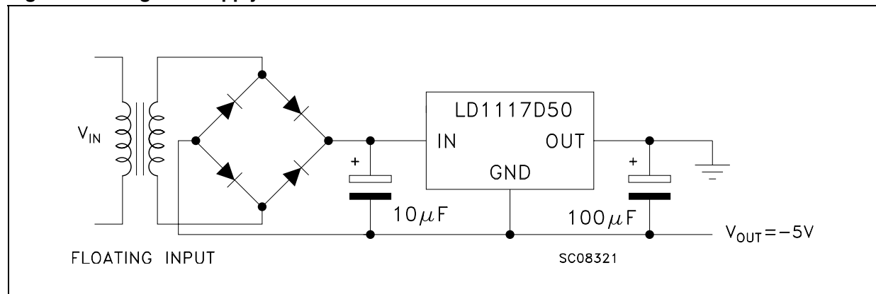
Figure 3. Negative supply
