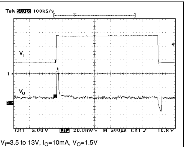
Figure 18. Line transient
