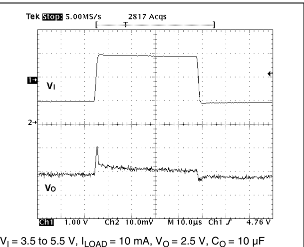
Figure 16. Line transient
