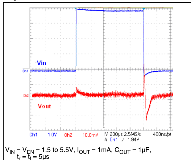
Figure 12. Line transient
