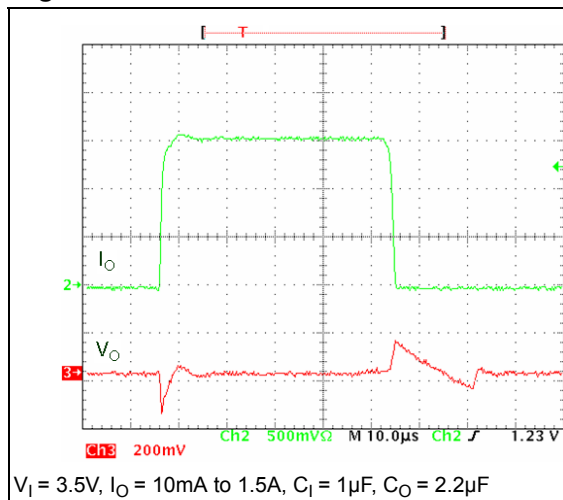
Figure 17. Load transient
