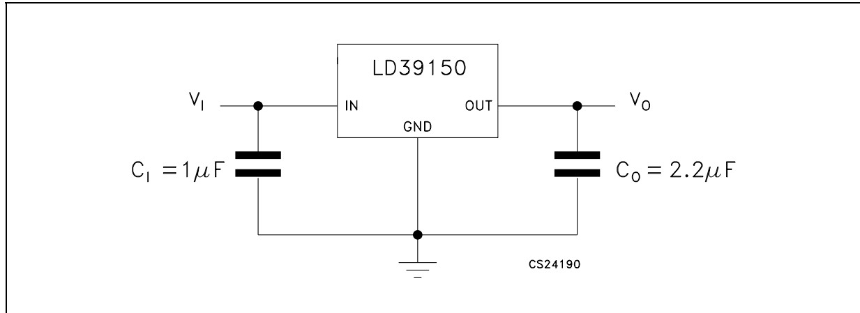
Figure 5. LD39150xx DPAK
