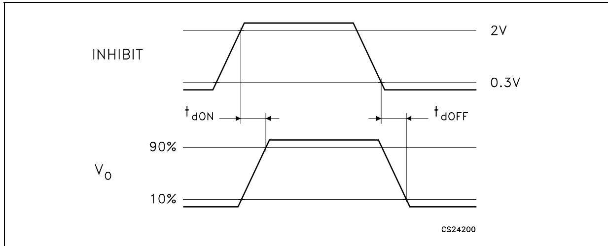
Figure 6. Timing diagram
