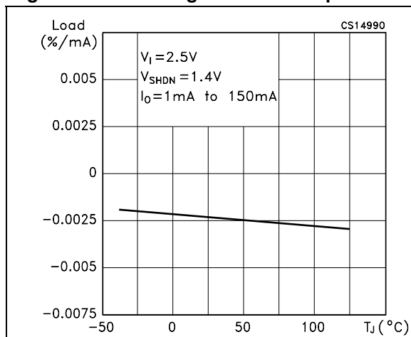
Figure 12. Load regulation vs temperature
