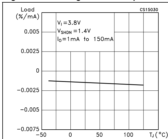
Figure 14. Load regulation vs temperature
