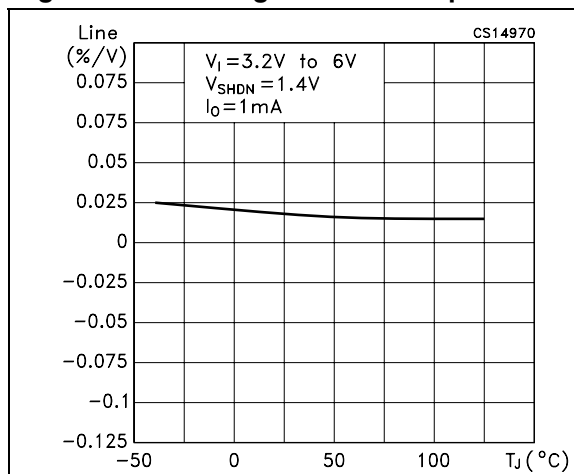
Figure 10. Line regulation vs temperature
