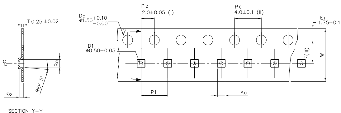
Figure 27. Tape dimensions
