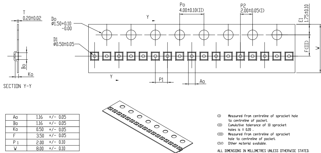
Figure 24. DFN4 1x1 tape outline
