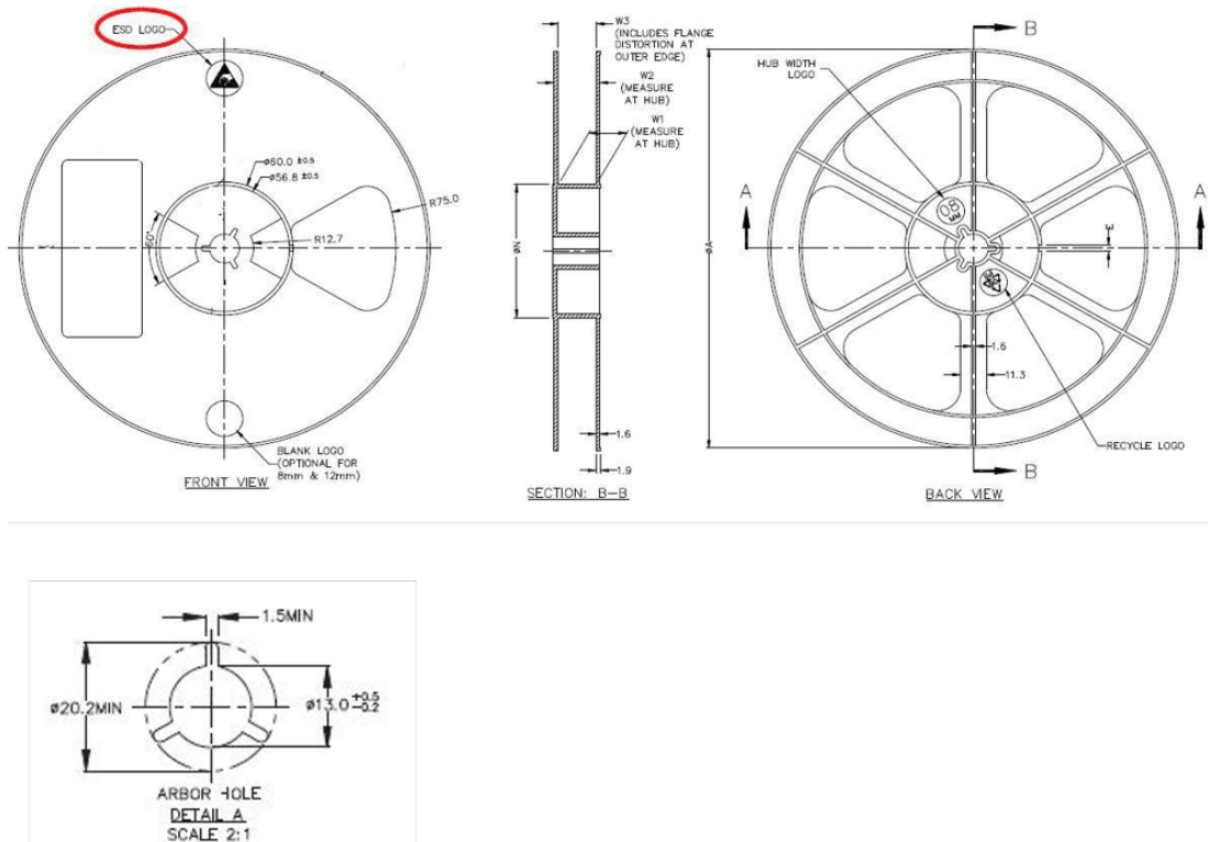
Figure 25. DFN4 1x1 reel outline
