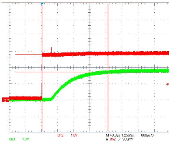
Figure 18. Turn-on Time ( V_{OUT} = 1.8\text{ V}; I_{OUT} = 0\text{ A} , V_{IN} = 2.8\text{ V} , t_r = t_f = 1\text{ }\mu\text{s} )
