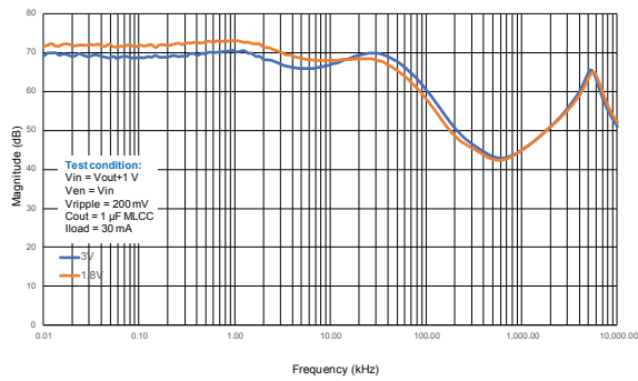
Figure 14. Supply voltage rejection vs. frequency
