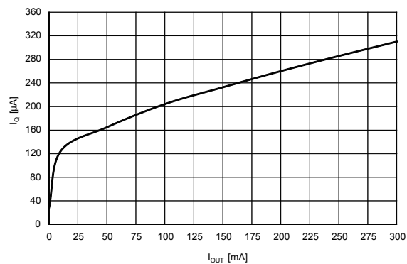
Figure 12. Quiescent current vs. output current ( V_{IN} = 2.8 V; V_{OUT} = 1.8 V)
