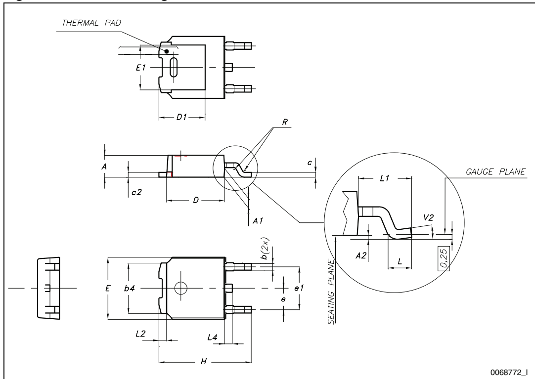
Figure 27. DPAK drawing
