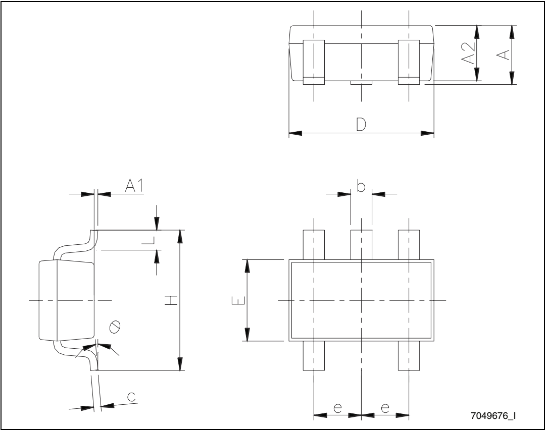
Figure 35. SOT23-5L drawing
