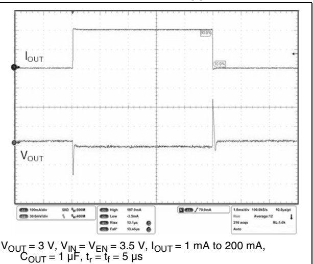
Figure 28. Load transient ( V_{OUT} = 3 V )
