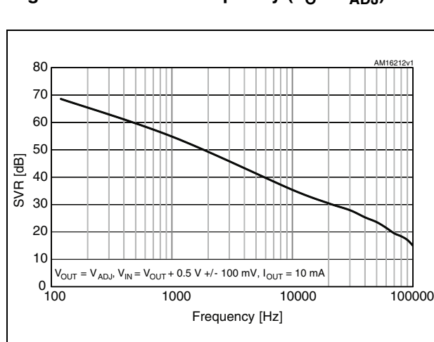
Figure 21. SVR vs. frequency ( V_O = V_{ADJ} )
