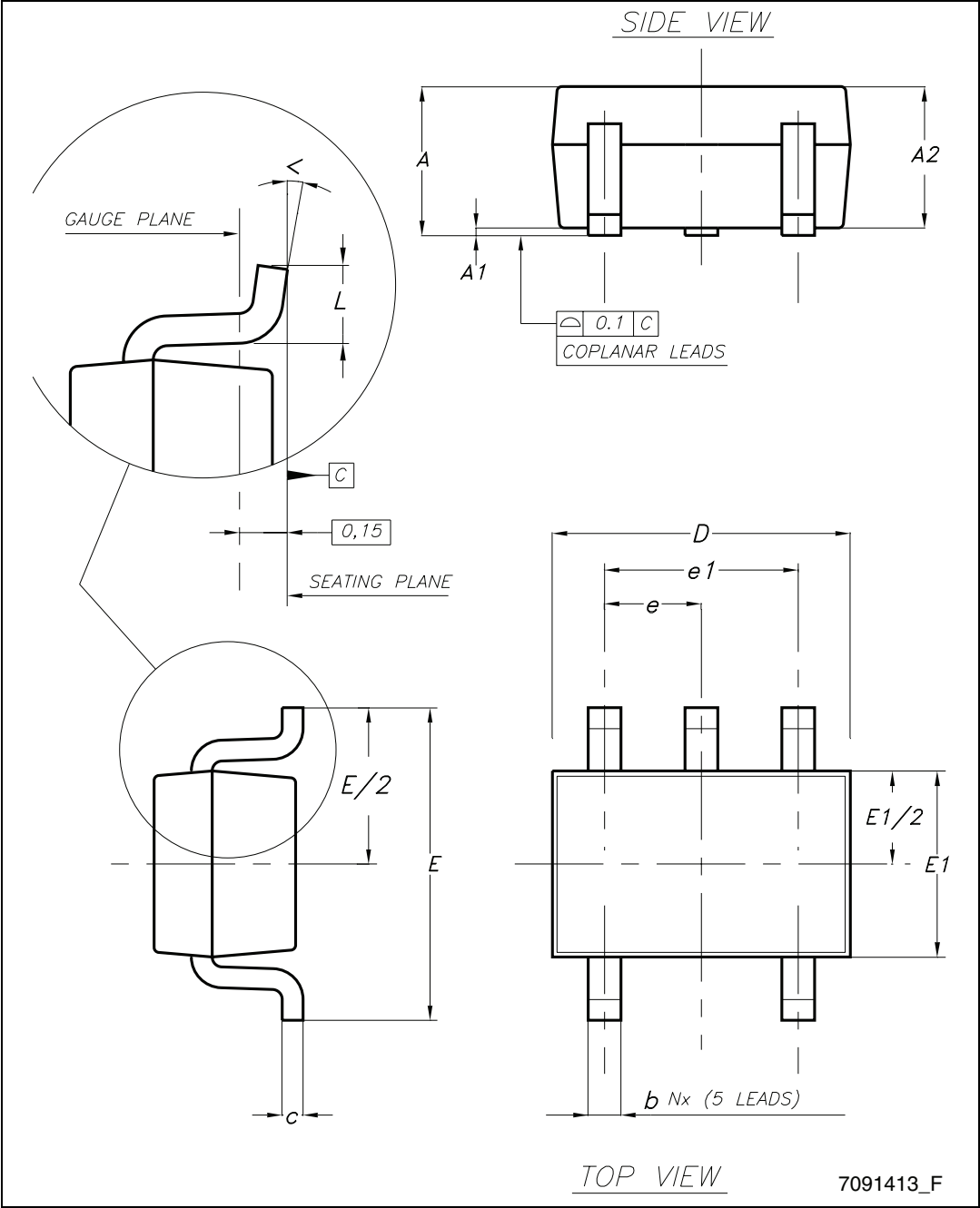
Figure 39. SOT323-5L drawing
