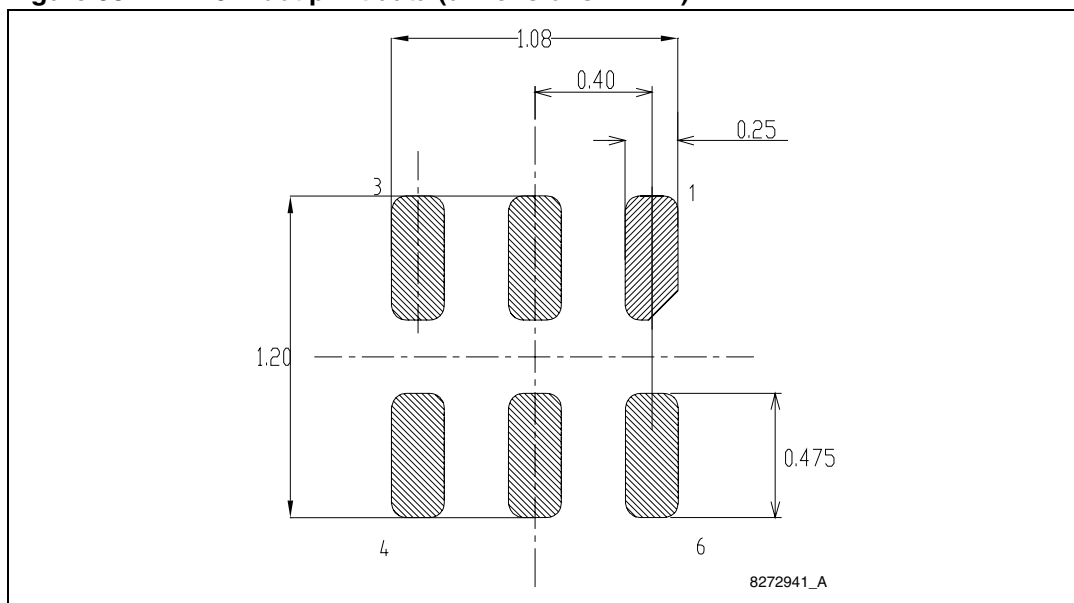
Figure 38. DFN6L foot print data (dimensions in mm)
