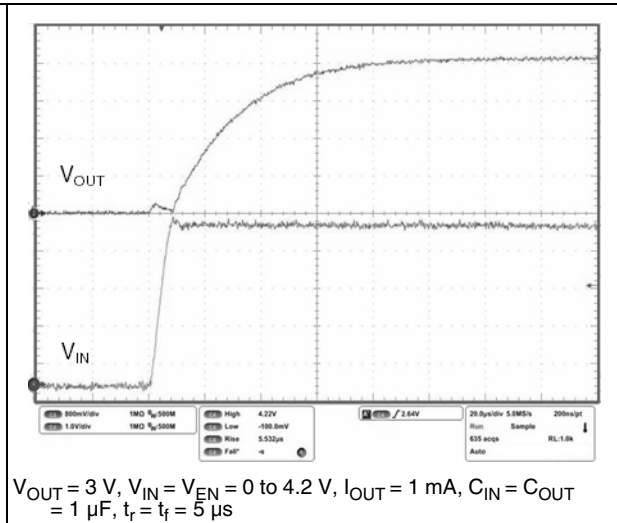
Figure 30. Startup transient
