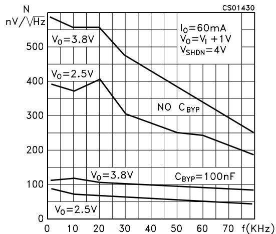
Figure 22: Spectrum Noise
