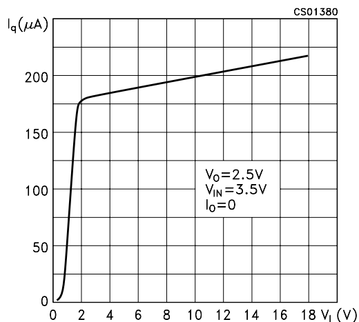
Figure 18: Quiescent Current vs Shutdown Voltage
