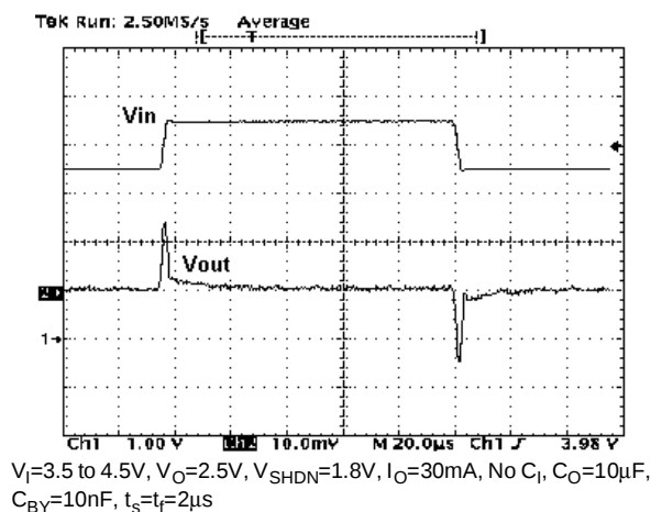
Figure 27: Line Transient
