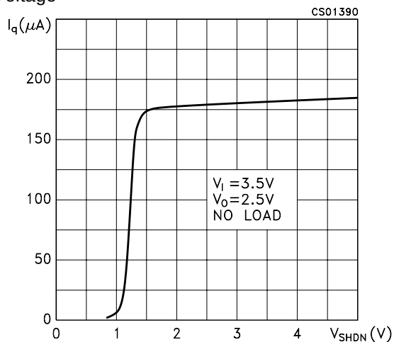
Figure 18: Quiescent Current vs Shutdown Voltage
