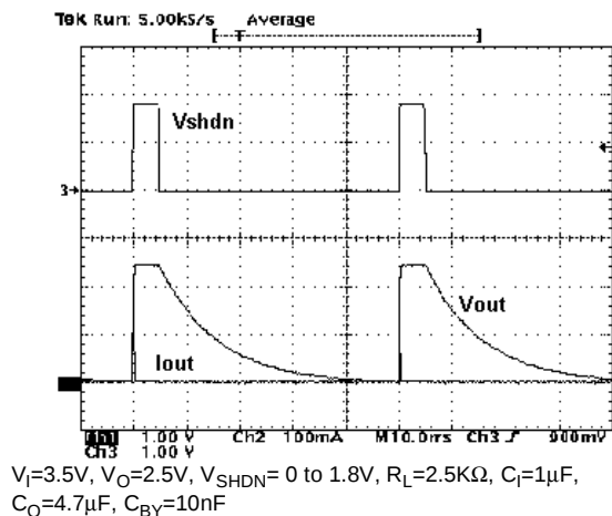
Figure 24: Start-up Transient
