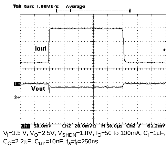
Figure 28: Load Transient
