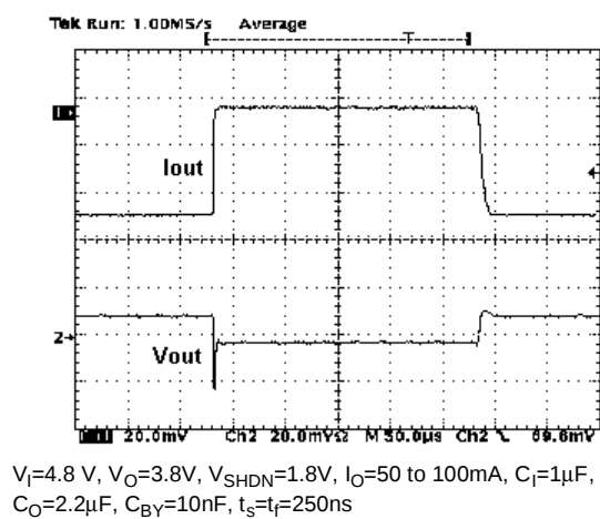
Figure 30: Load Transient
