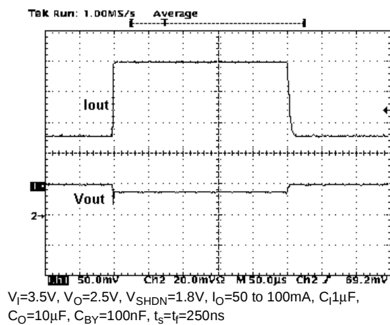
Figure 29: Load Transient
