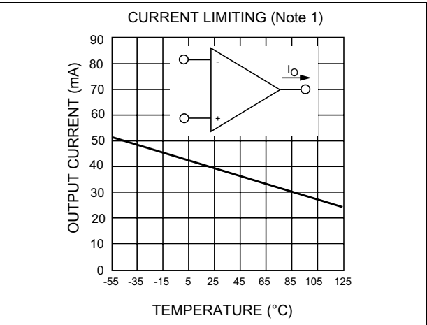
Figure 8. Current limiting
