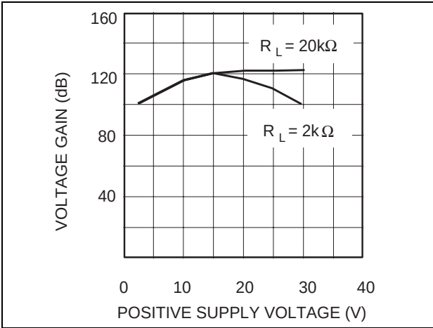
Figure 15. Positive supply voltage
