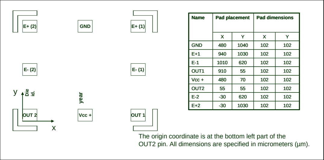
Figure 2. Pad locations
