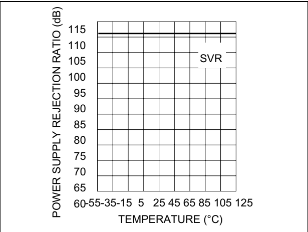
Figure 18. Power supply rejection ratio
