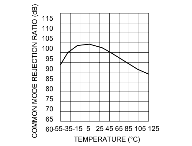
Figure 20. Common mode rejection ratio
