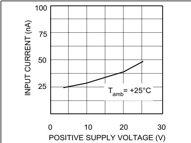
Figure 17. Positive supply voltage
