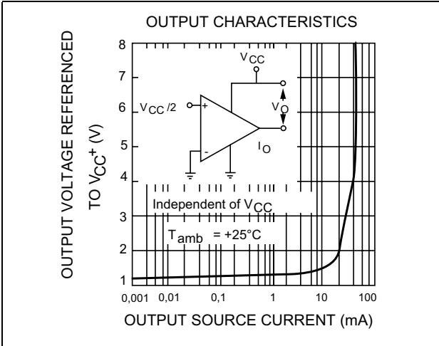
Figure 11. Output characteristics
