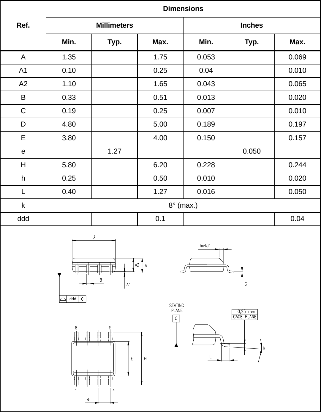
Figure 21. SO-8 package
