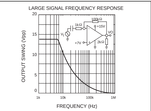
Figure 4. Large signal frequency response
