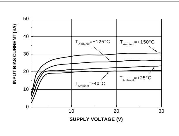
Figure 6. Supply voltage
