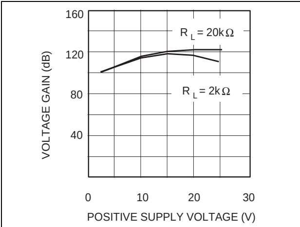
Figure 19. Positive supply voltage
