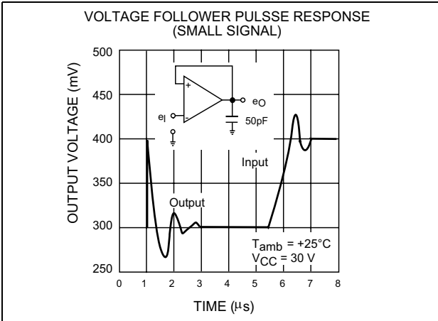
Figure 9. Voltage follower pulse response
