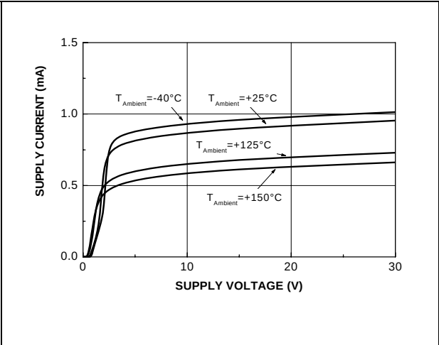
Figure 12. Supply voltage
