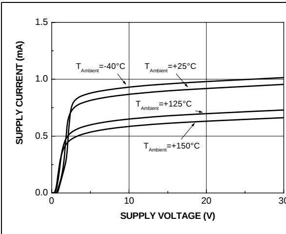
Figure 7. Supply current
