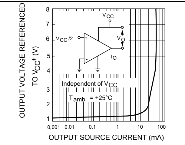
Figure 8. Output characteristics
