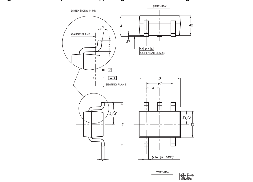
Figure 34. SC70-5 (or SOT323-5) package mechanical drawing
