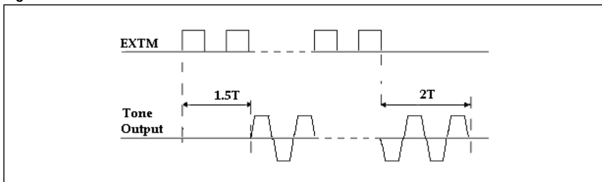
Figure 2. EXTM waveform
