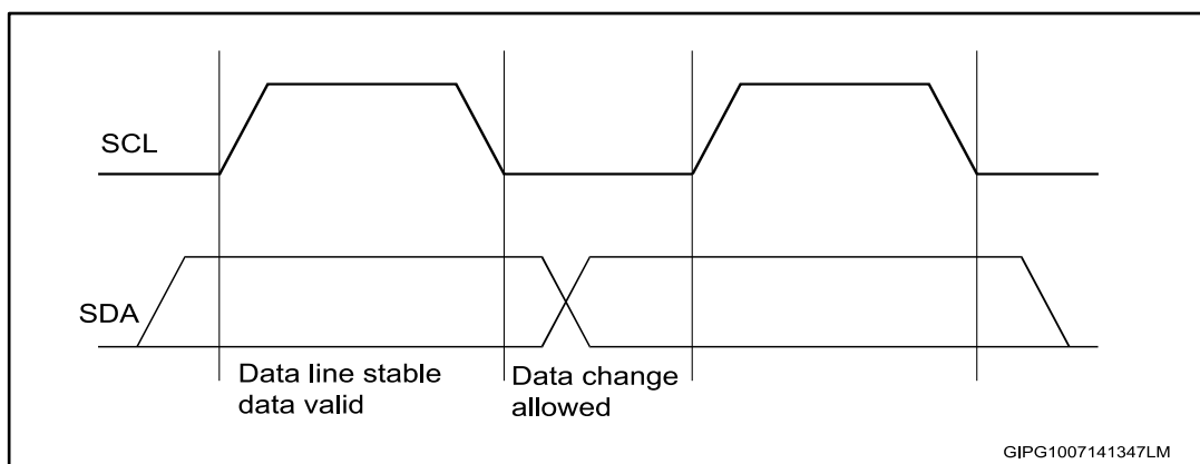
Figure 9: Timing diagram of I 2 C bus
