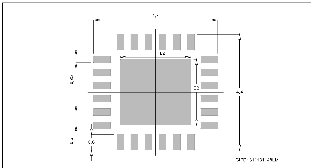
Figure 15: QFN24L (4x4) footprint recommended data (mm)
