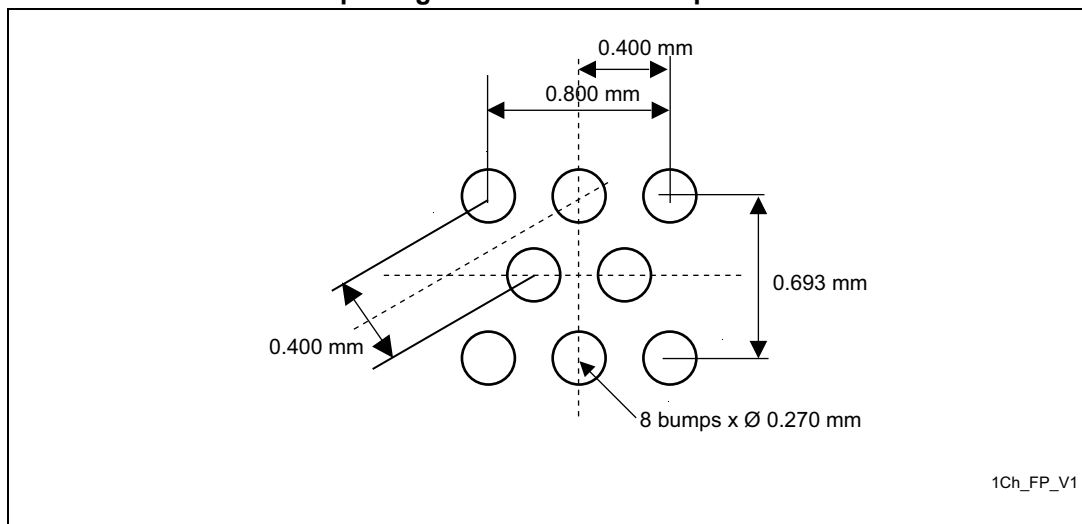
Figure 22. WLCSP - 8-bump, 1.289 x 1.099 mm, 0.4 mm pitch wafer level chip scale package recommended footprint
