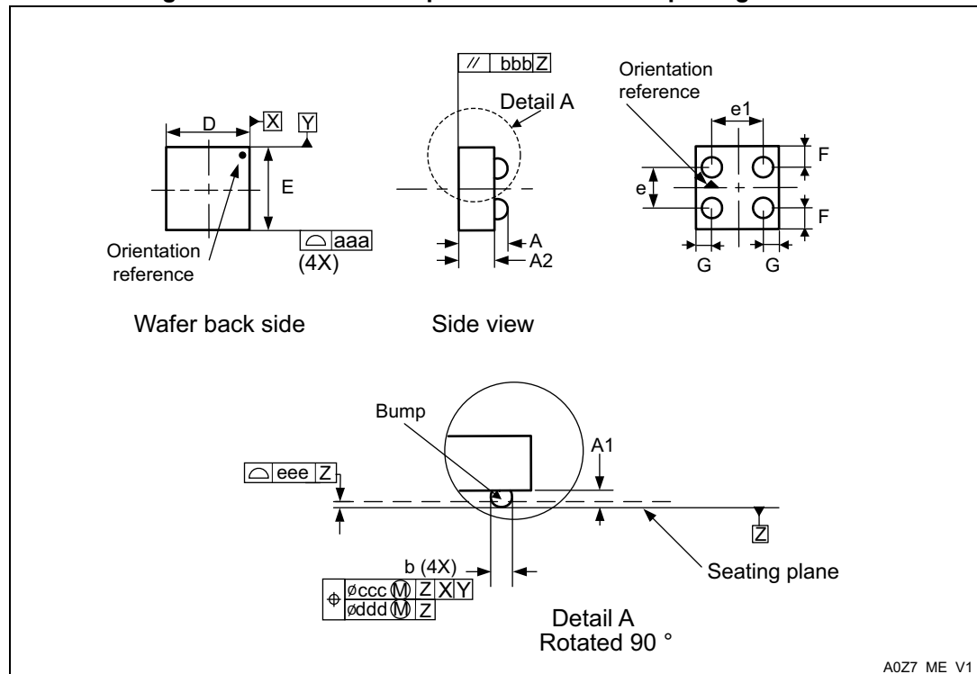
Figure 12. WLCSP 4-bump M24C32S-FCU6T/T package outline
