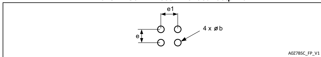
Figure 15. WLCSP package with Back Side Coating (BSC) M24C32S-FCU6T/TF recommended footprint
