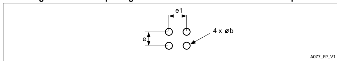
Figure 13. WLCSP package M24C32S-FCU6T/T recommended footprint
