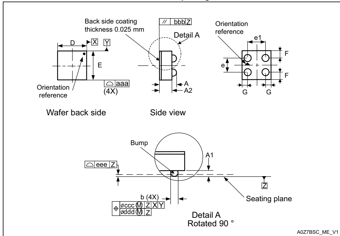
Figure 14. WLCSP 4-bump ultra-thin with Back Side Coating (BSC) M24C32S-FCU6T/TF package outline
