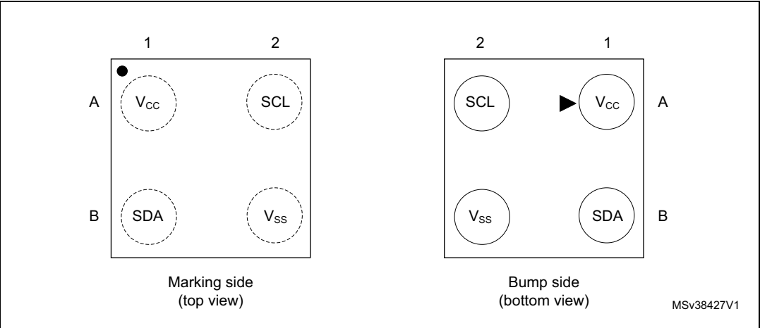
Figure 2. 4-bump WLCSP connections (top view, marking side, with balls on the underside)
