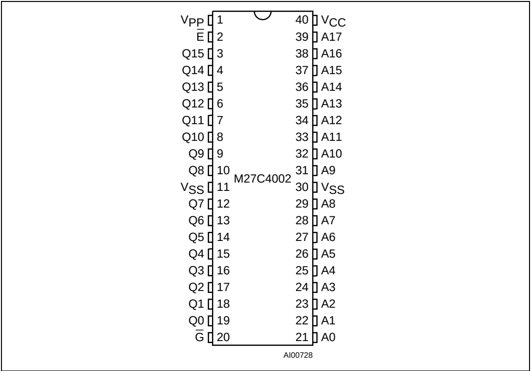
Figure 2. DIP Connections
