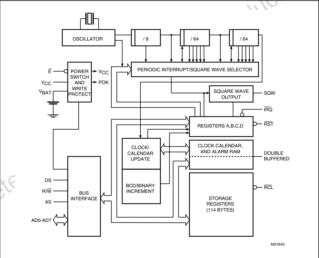
Figure 4. Block diagram
