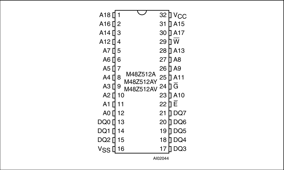
Figure 2. DIP connections
