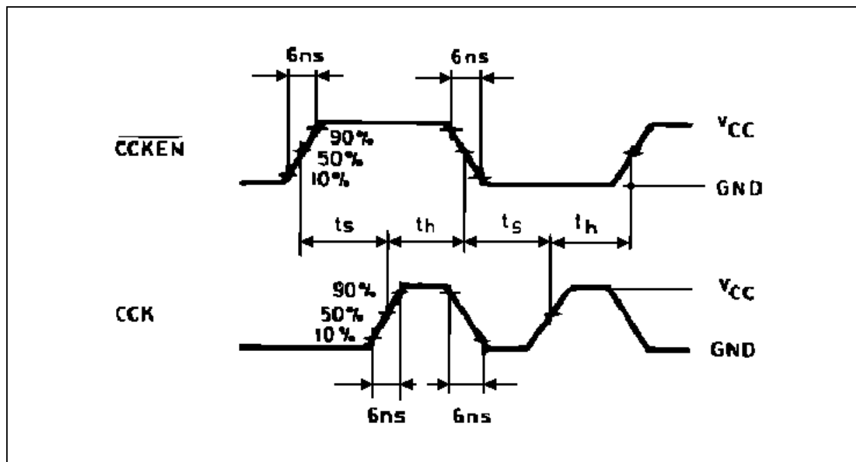
WAVEFORM 4 : MINIMUM SETUP AND HOLD TIME ( f=1\text{MHz} ; 50% duty cycle)
