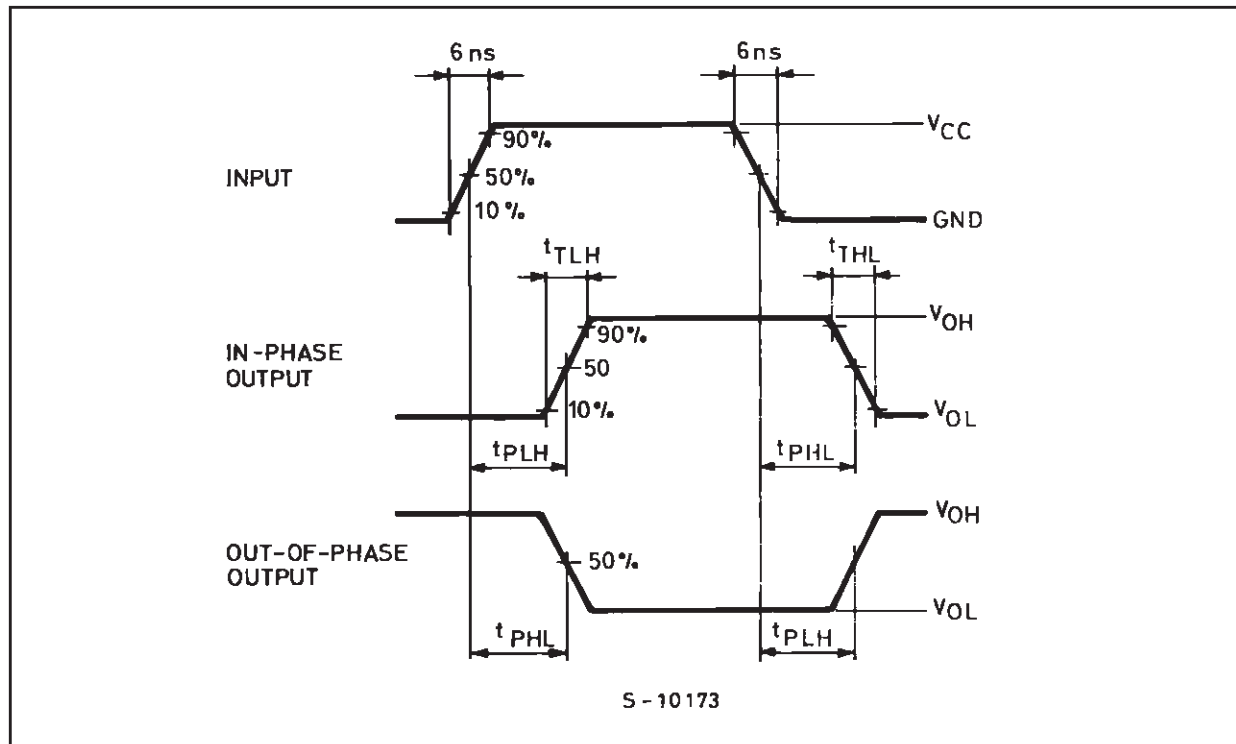
WAVEFORM : PROPAGATION DELAY TIME ( f=1\text{MHz} ; 50% duty cycle)
