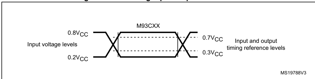
Figure 9. AC testing input output waveforms
