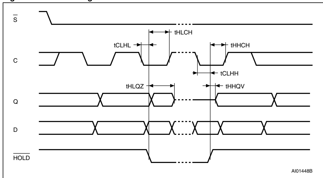
Figure 16. Hold timing
