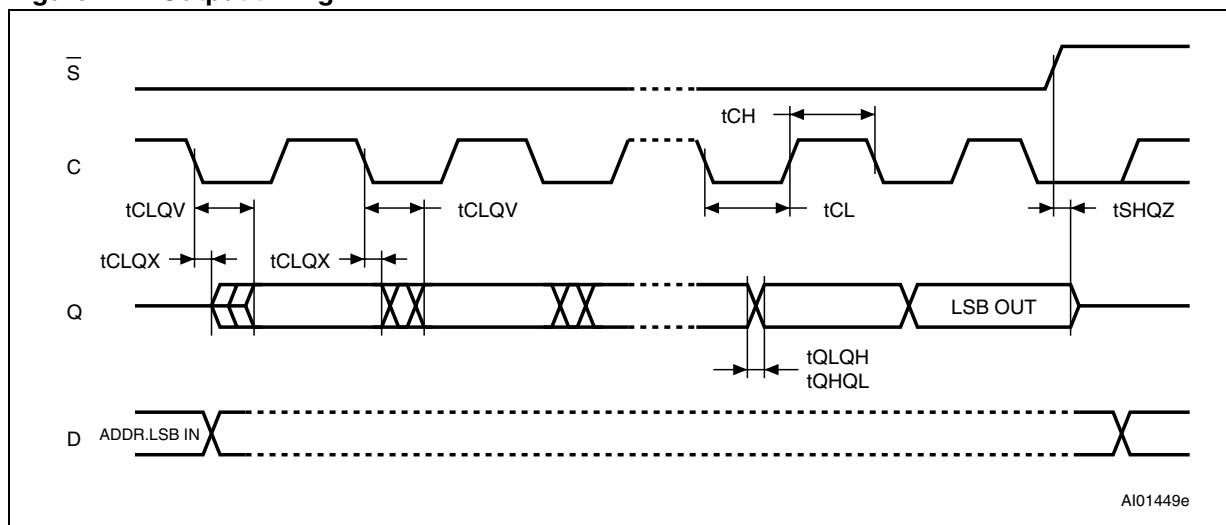
Figure 17. Output timing
