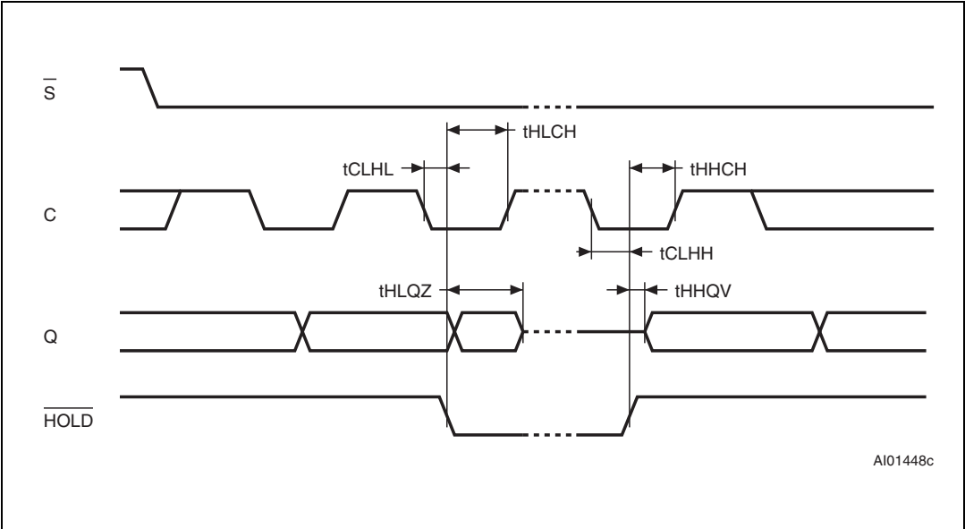
Figure 20. Hold timing
