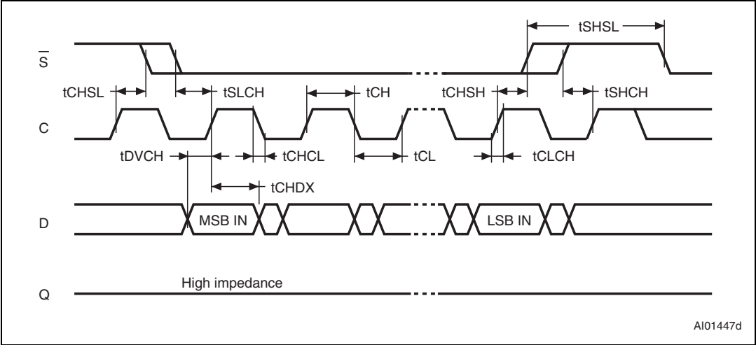
Figure 19. Serial input timing
