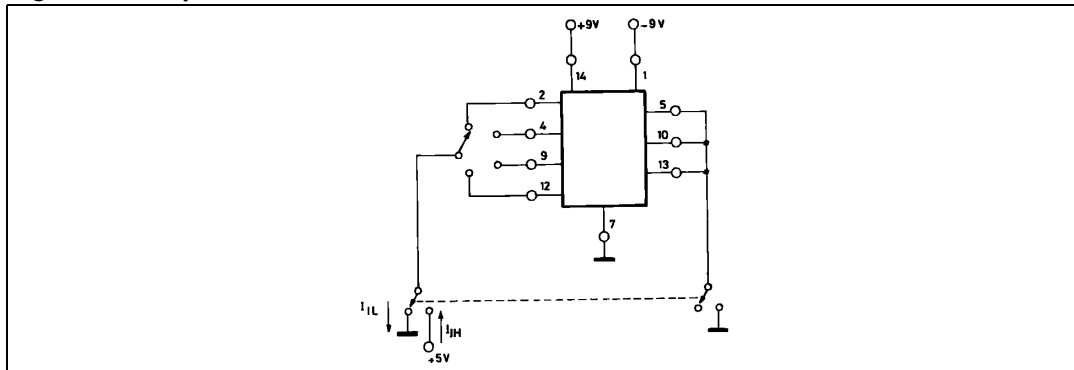
Figure 3. Input current
