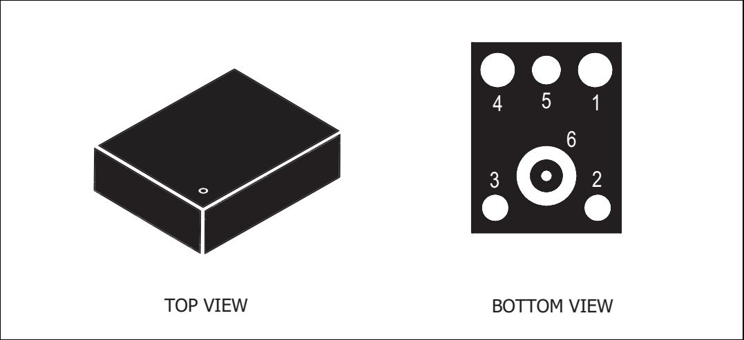
Figure 1. Pin connections
