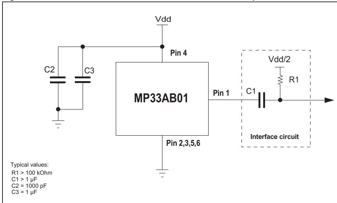
Figure 3. MP33AB01 electrical connections and external component values
