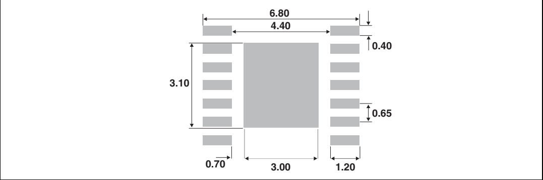
Figure 16. Footprint (dimensions in mm)
