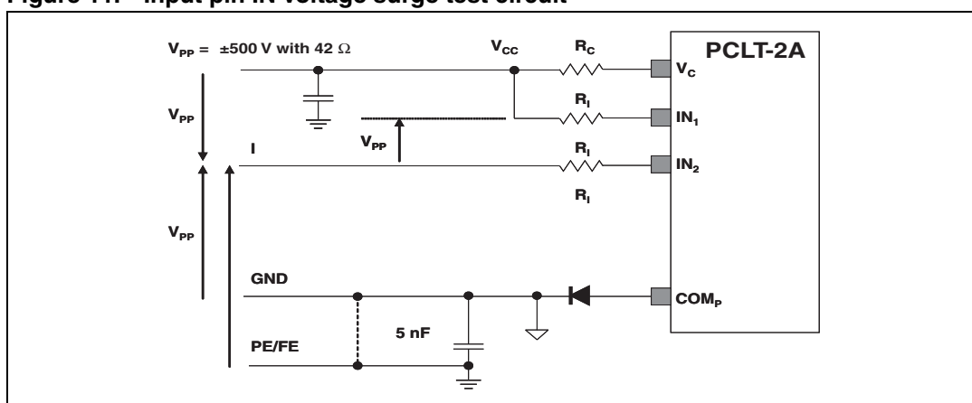
Figure 11. Input pin IN voltage surge test circuit
