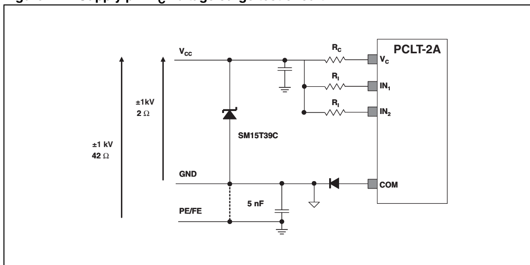
Figure 12. Supply pin V_C voltage surge test circuit
