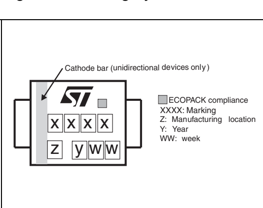
Figure 18. Marking layout (1)
