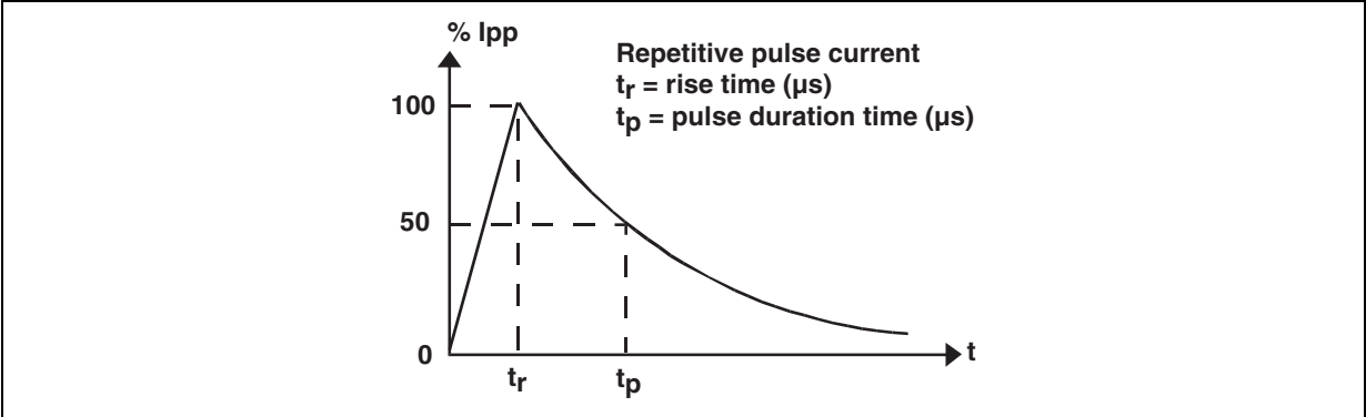
Figure 2. Pulse form
