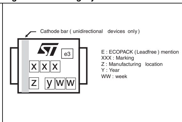
Figure 14. Marking layout
