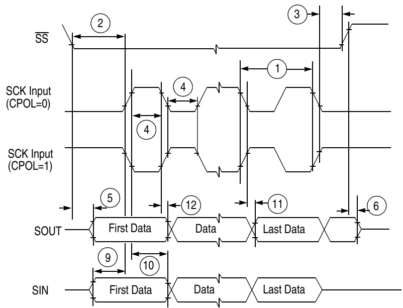
Figure 32. DSPI classic SPI timing — master, CPHA = 1
