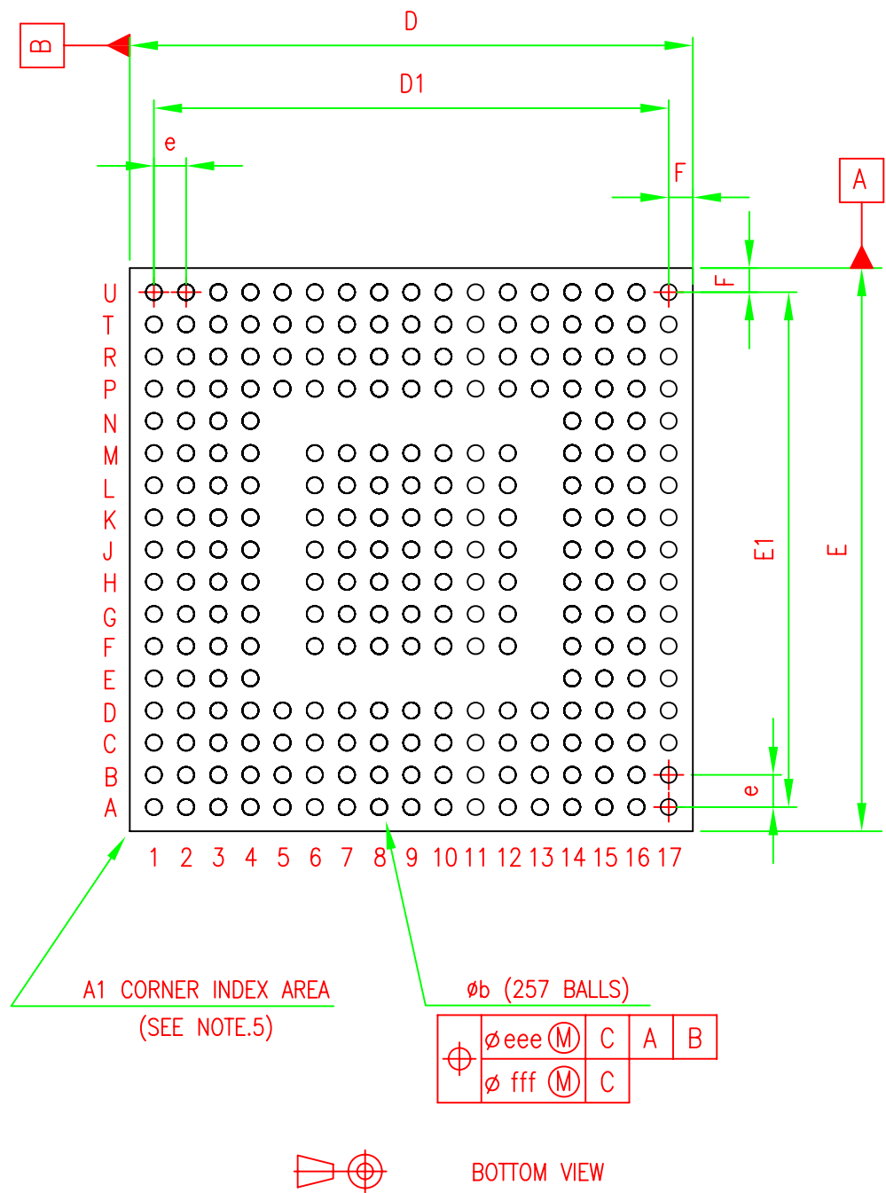
Figure 42. LFBGA257 package mechanical drawing
