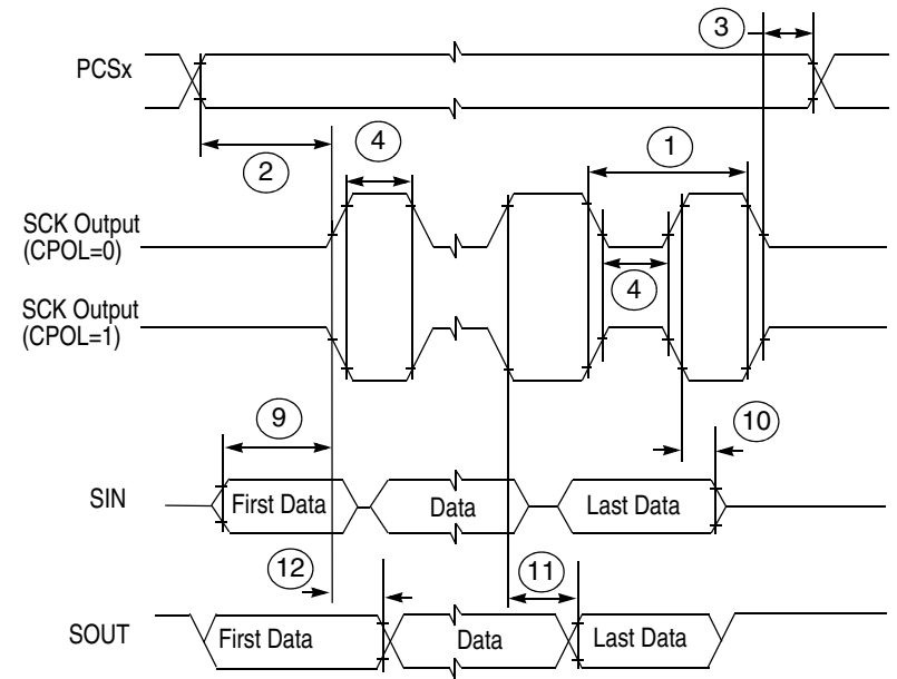
Figure 34. DSPI classic SPI timing — slave, CPHA = 1
