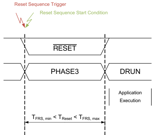
Figure 17. Functional Reset Sequence Short
