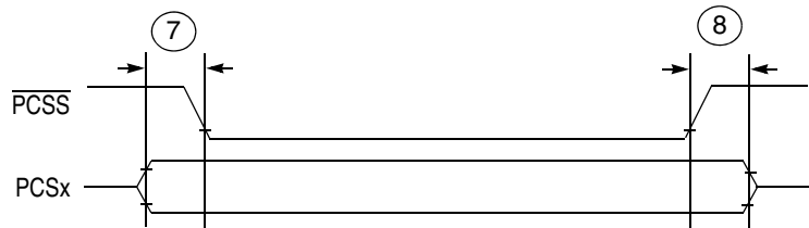
Figure 38. DSPI modified transfer format timing — slave, CPHA = 1
