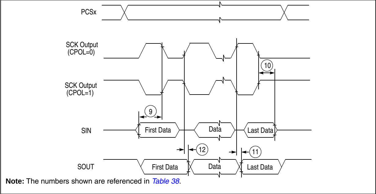
Figure 30. DSPI classic SPI timing — master, CPHA = 1
