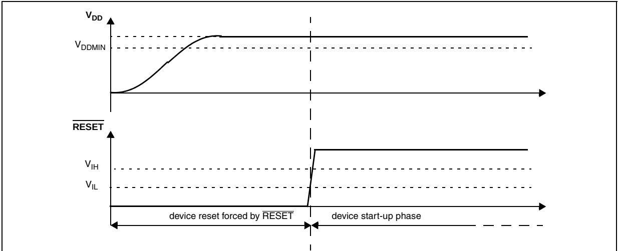
Figure 20. Start-up reset requirements
