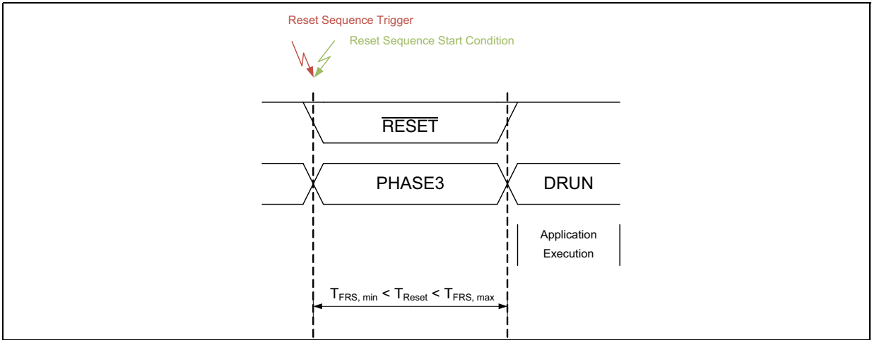
Figure 16. Functional Reset Sequence Short
