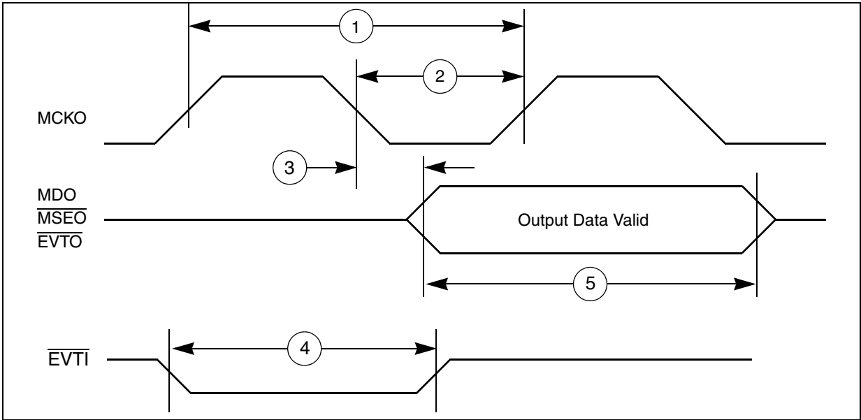
Figure 25. Nexus output timing
