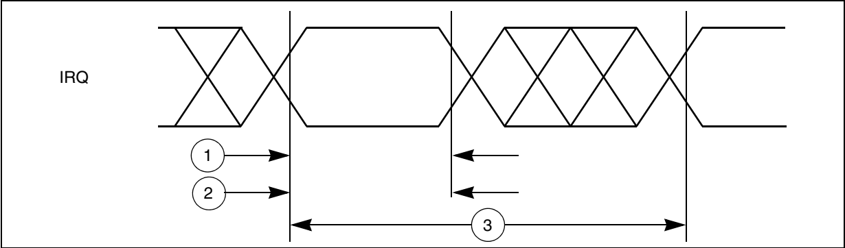
Figure 28. External interrupt timing
