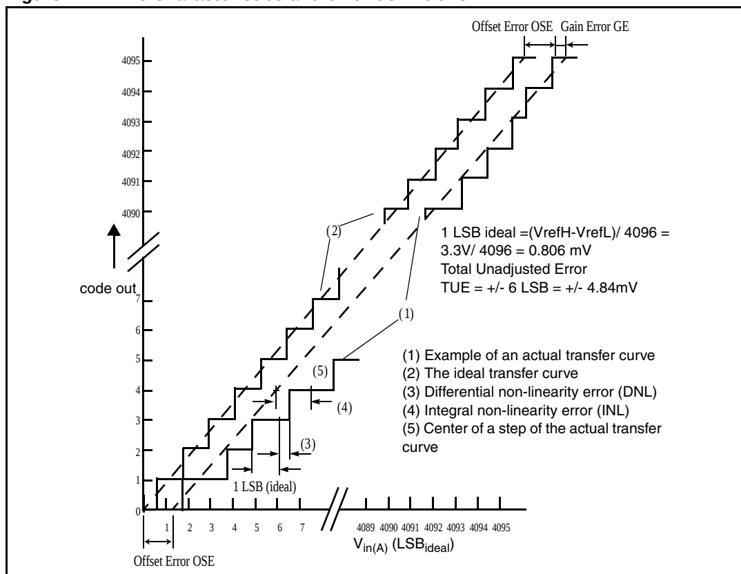
Figure 7. ADC characteristics and error definitions
