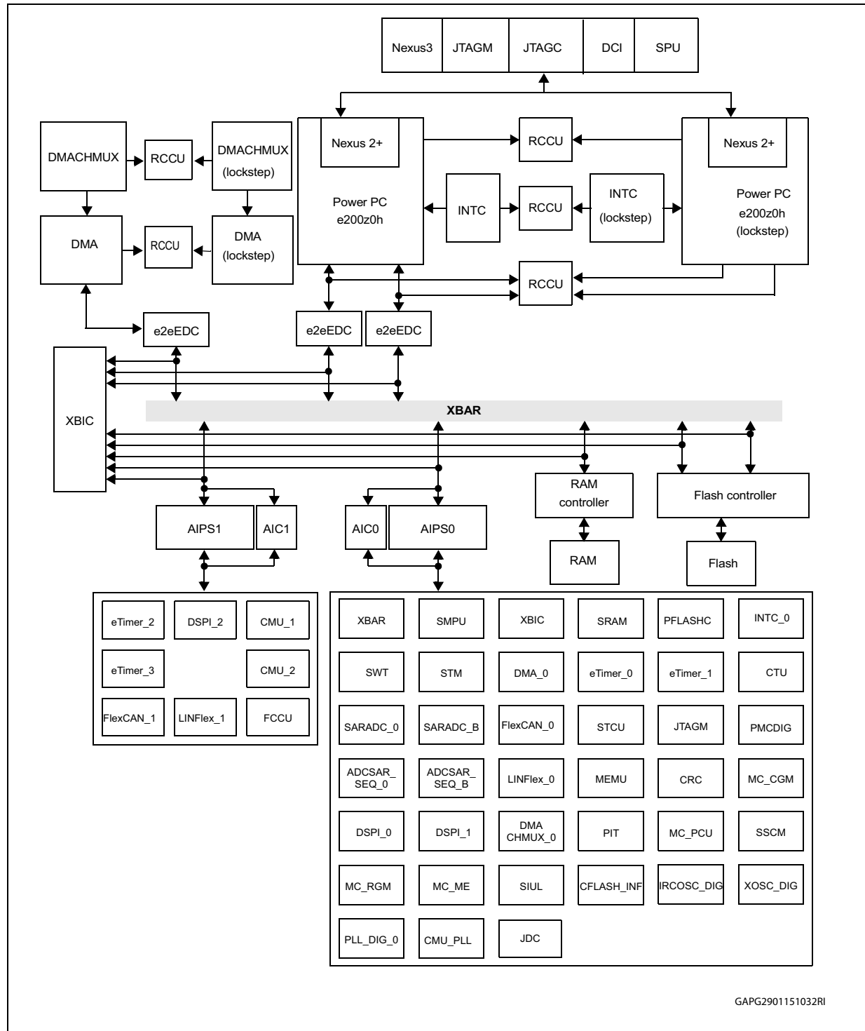
Figure 1. Family Superset block diagram
