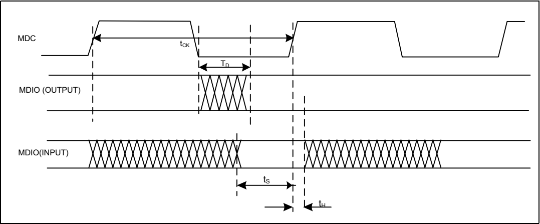
Figure 21. MDC waveforms
