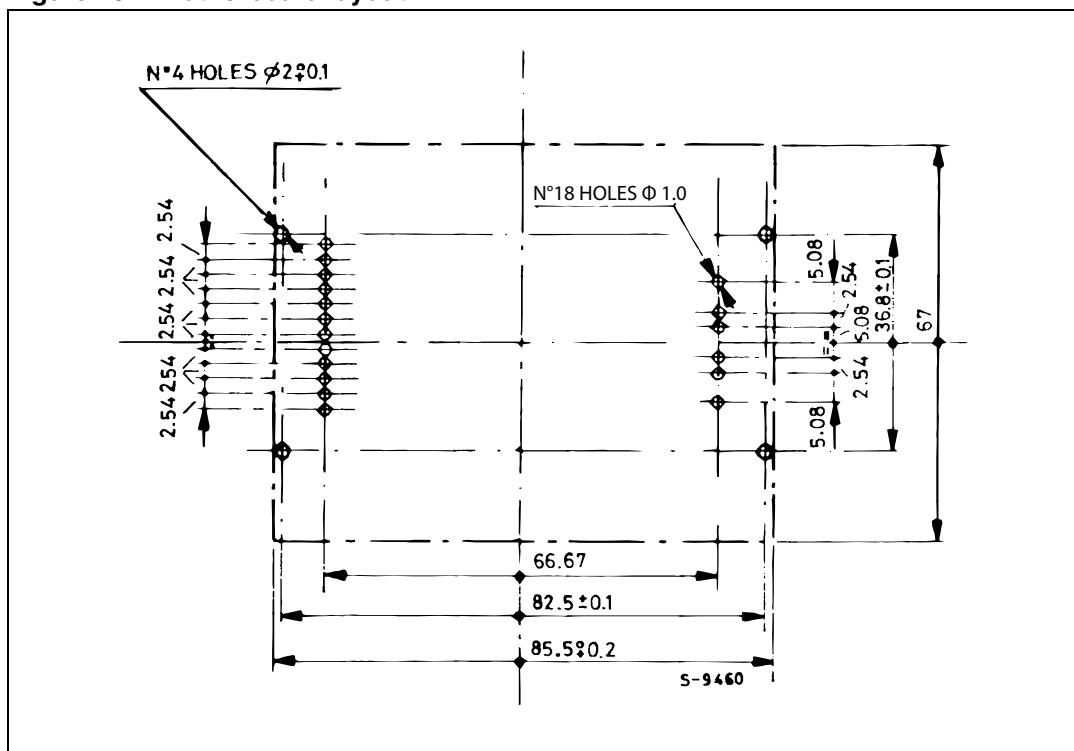
Figure 20. Motherboard layout
