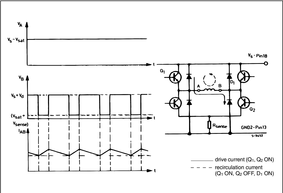
Figure 12. Chopper control with slow decay
