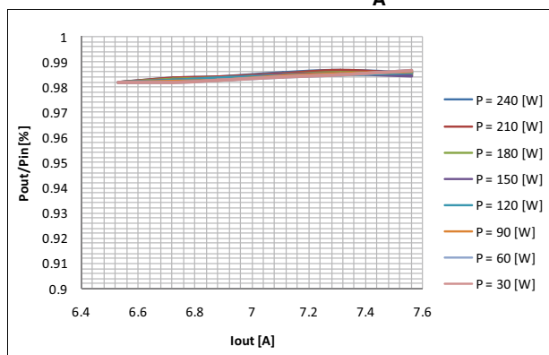
Figure 10. Power efficiency measured on the board ISV009v1 at T_A=25^\circ\text{C}
