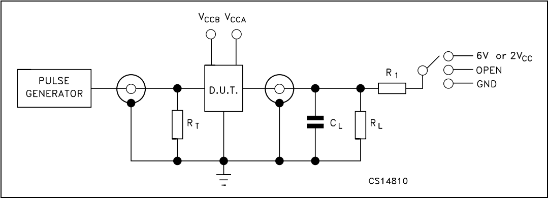
Figure 4. Test circuit
