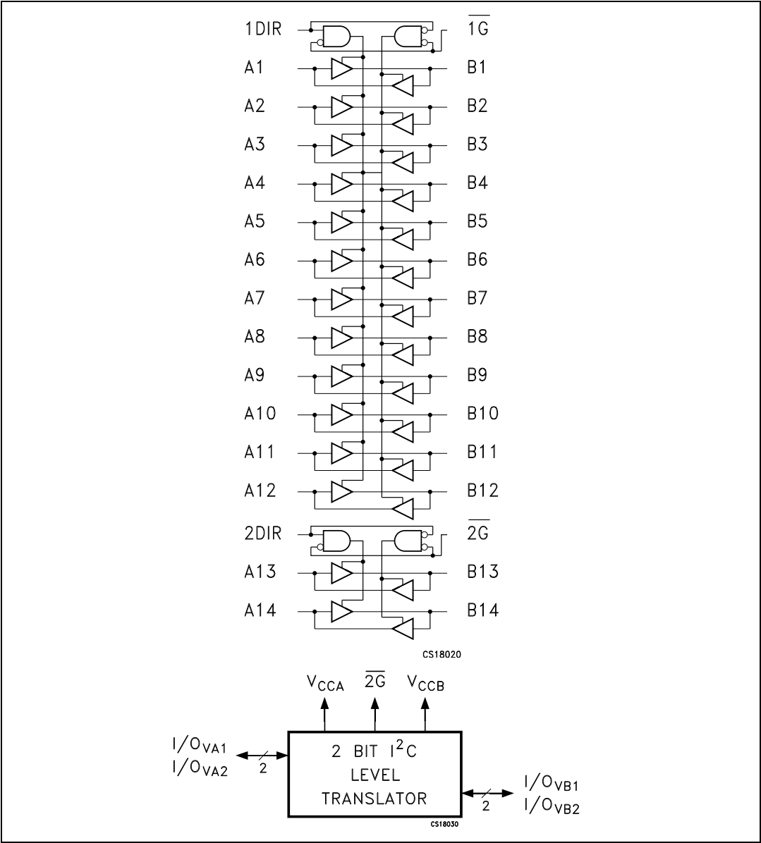
Figure 1. Logic diagram
