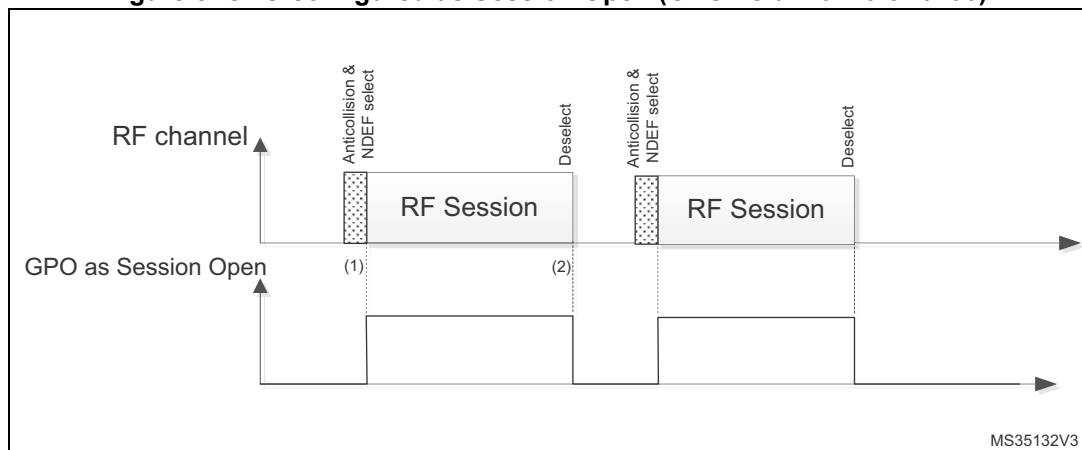
Figure 5. GPO configured as Session Open (GPO field = 0x10 or 0x90)
