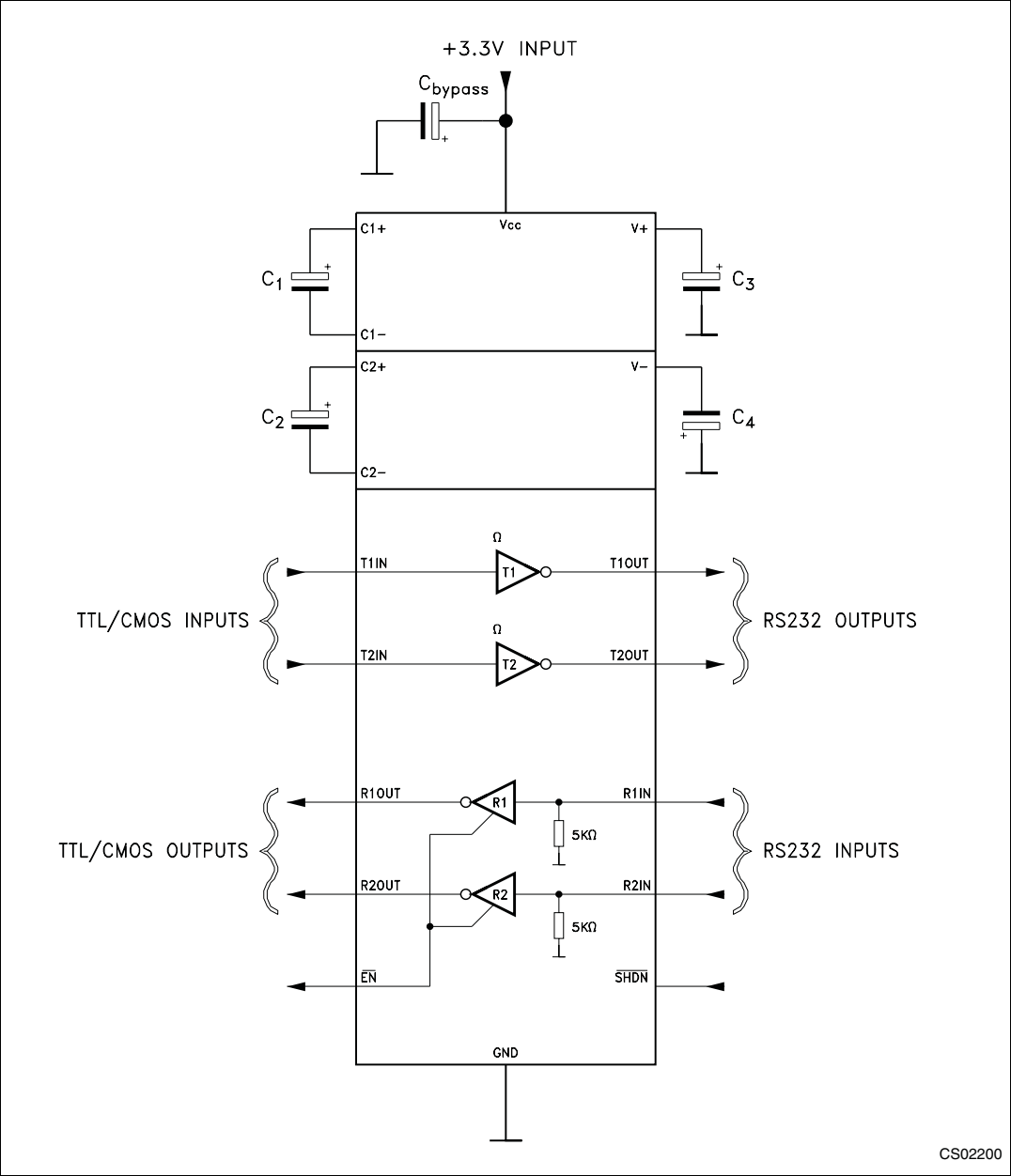
Figure 2. Application circuits
