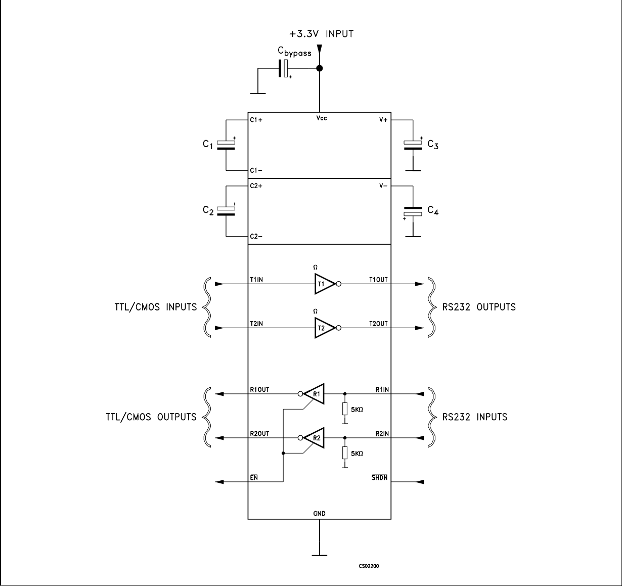
Figure 2. Application schematic
