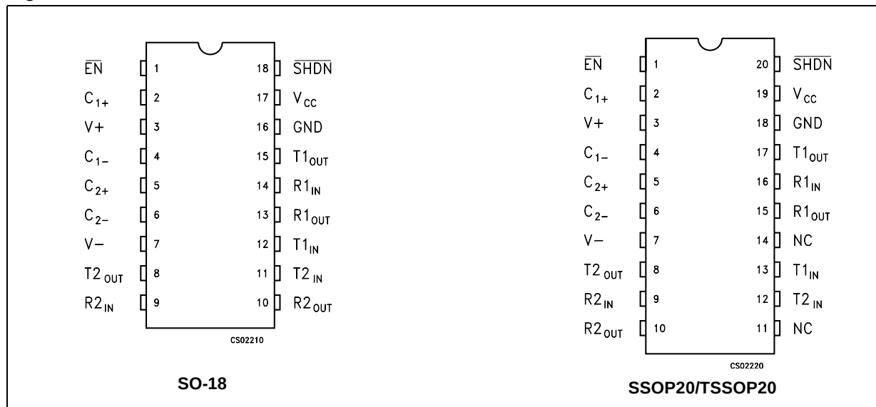
Figure 1. Pin connection
