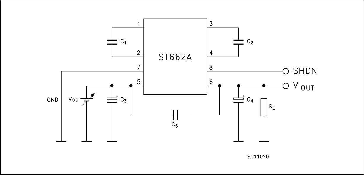
Figure 11. Test circuit
