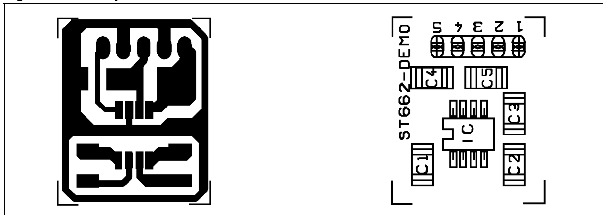
Figure 15. KIT layout
