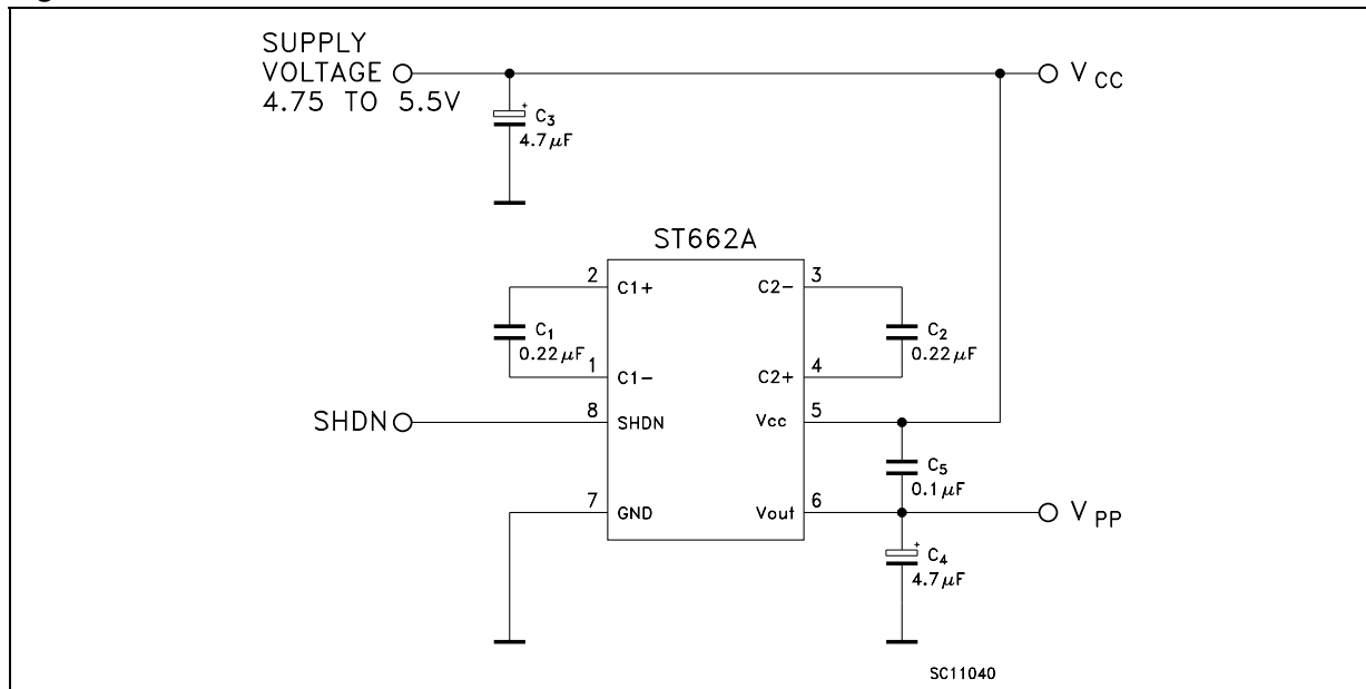
Figure 16. Electrical schematic
