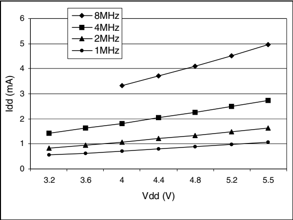
Figure 72. Typ. I DD in Slow-wait mode
