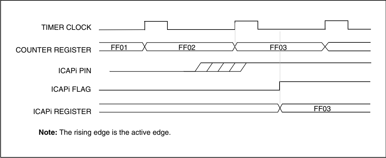
Figure 44. Input Capture Timing Diagram
