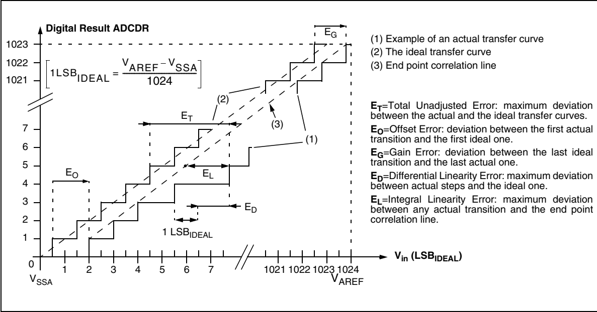
Figure 95. ADC Accuracy Characteristics
