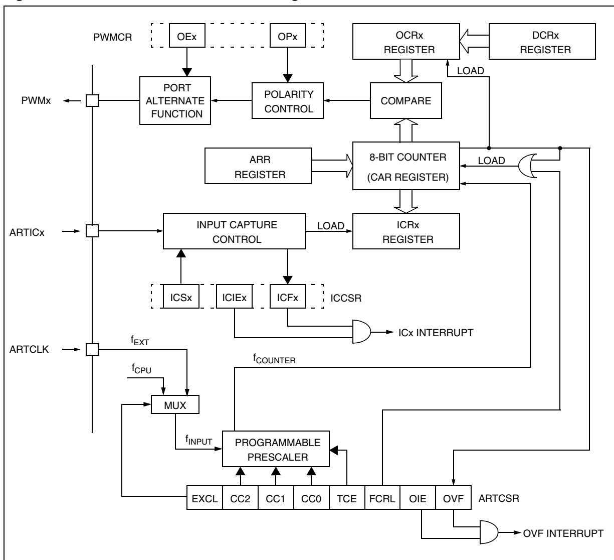
Figure 33. PWM Auto-Reload Timer Block Diagram
