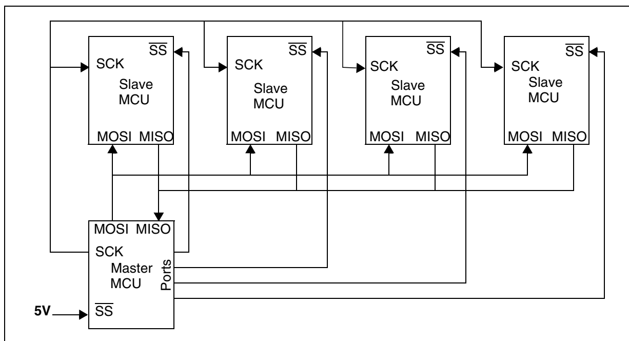
Figure 56. Single Master / Multiple Slave Configuration
