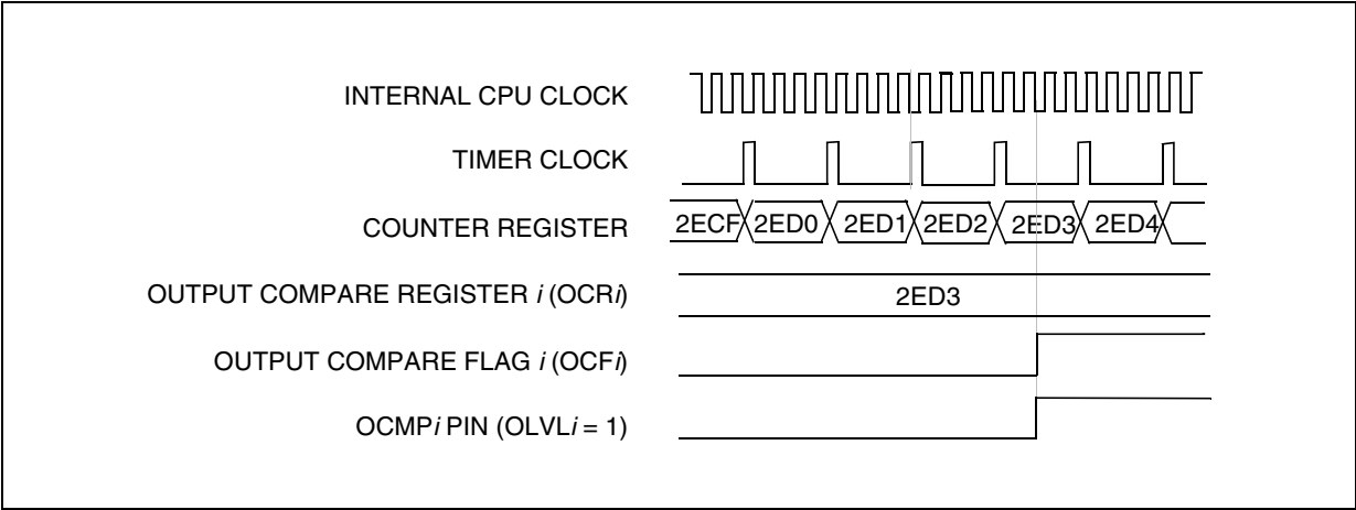
Figure 47. Output Compare Timing Diagram, f_{\text{TIMER}} = f_{\text{CPU}}/4
