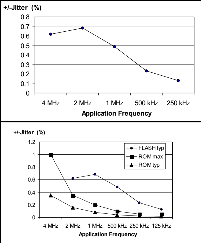
Figure 75. Integrated PLL Jitter vs signal frequency 1
