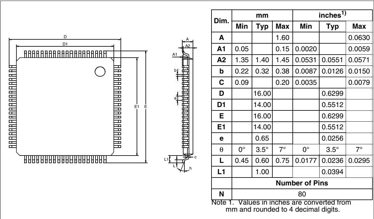
Figure 96. 80-Pin Low Profile Quad Flat Package
