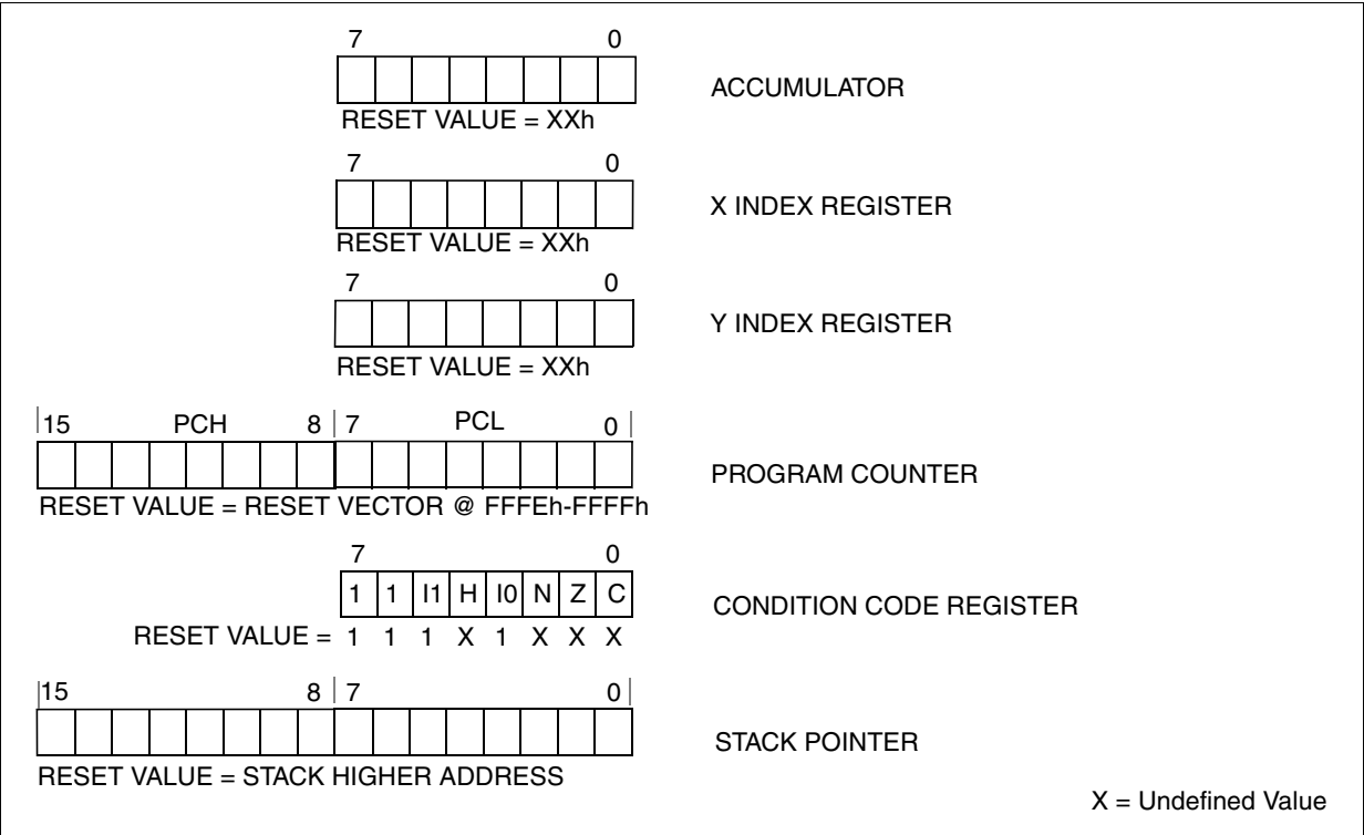
Figure 9. CPU Registers
